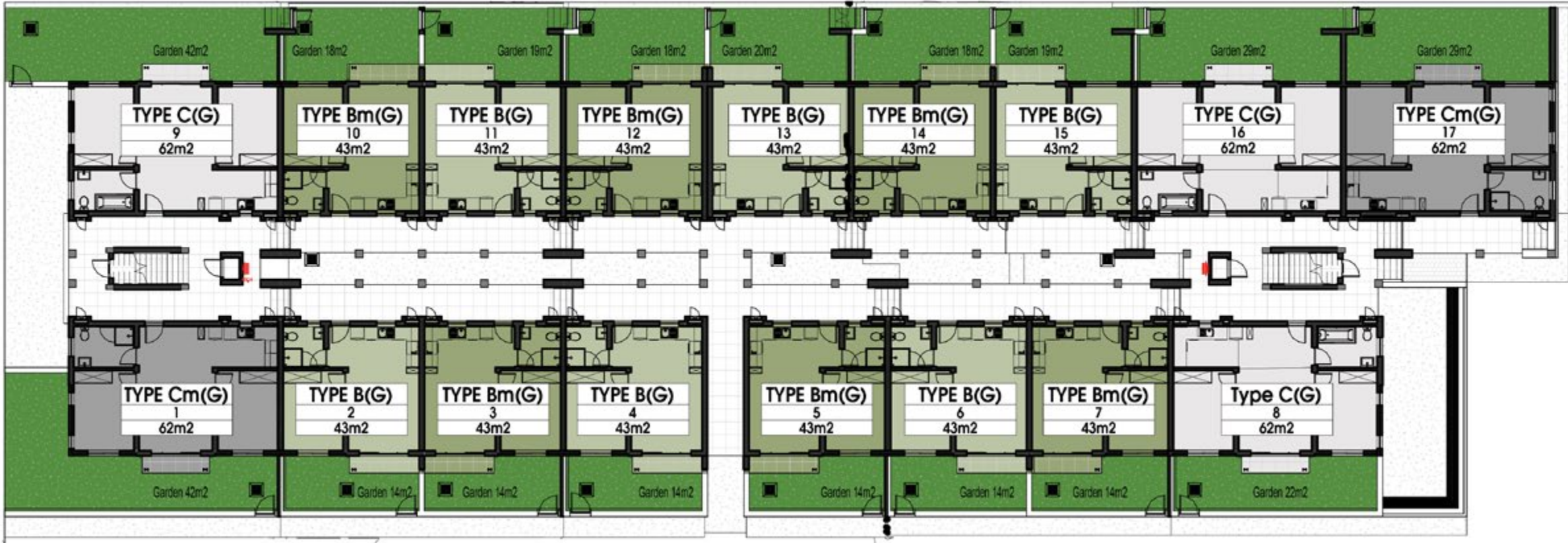
GROUND FLOOR
