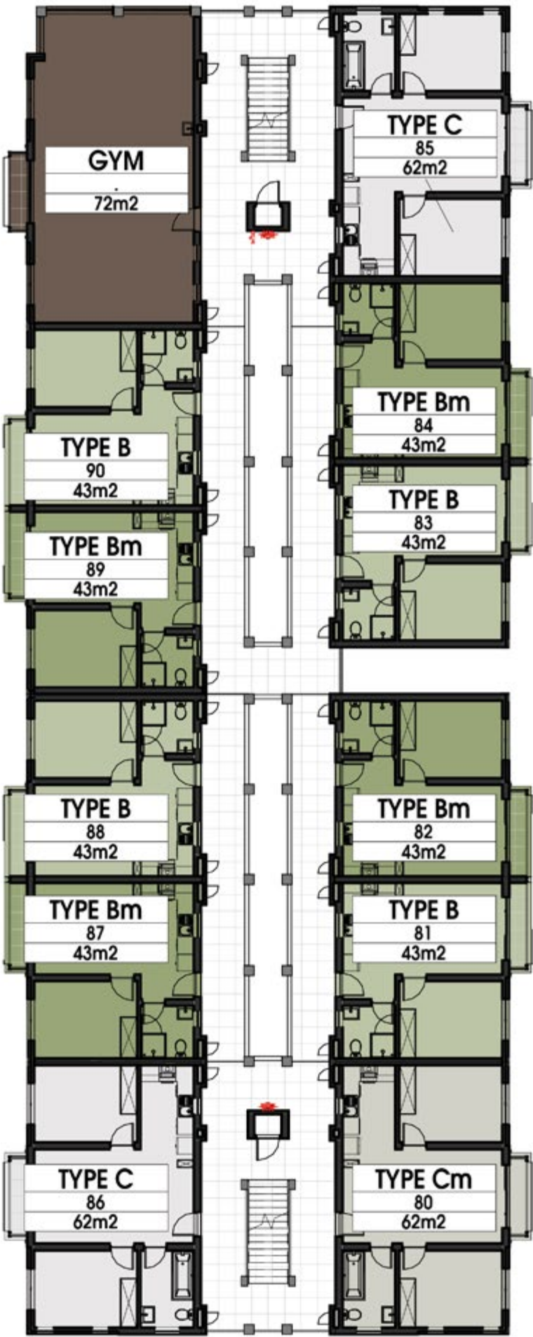
FIRST FLOOR
